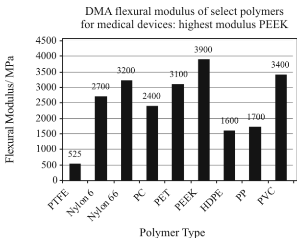
Fig. 10 DMA flexural modulus of polymers for medical devices
